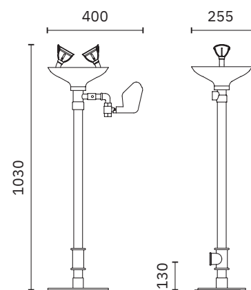
Emergency eyewasher with pedestal
