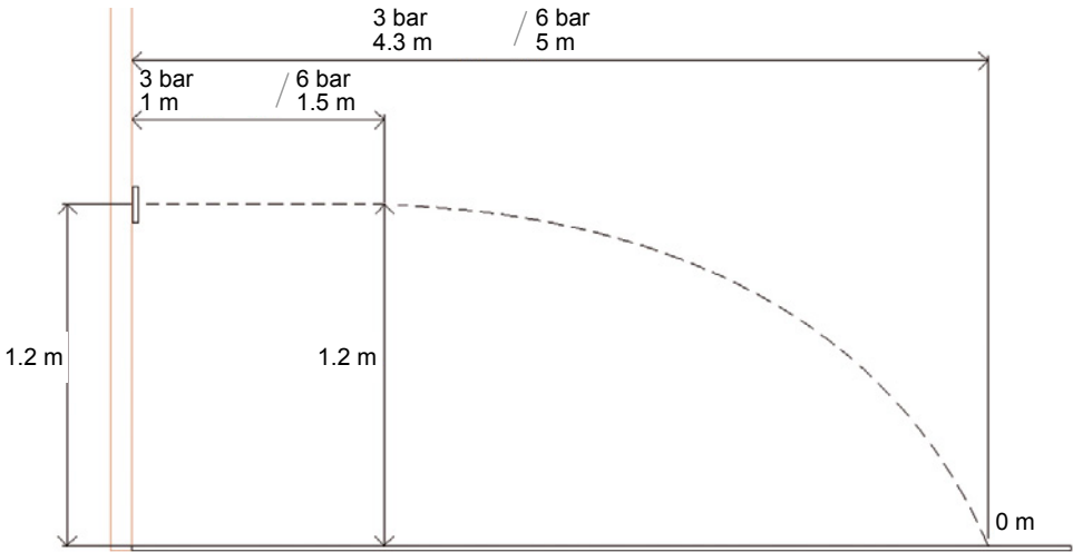
Whirlpool jet performance.
