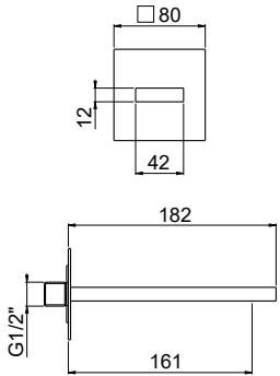
Wall-mounted washbasin/bathtub spout
