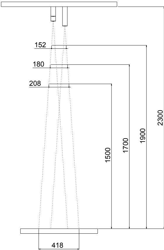
Ceiling-mounted
