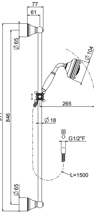
ART. 84220/71-CR Colonial shower 1 jet ART. 84020/71-CR Old America shower 1 jet
