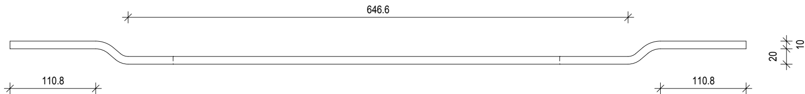
Frontansicht Front view
